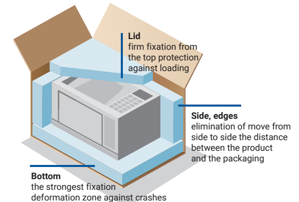
Form deformation zones: use fixing and filling materials
