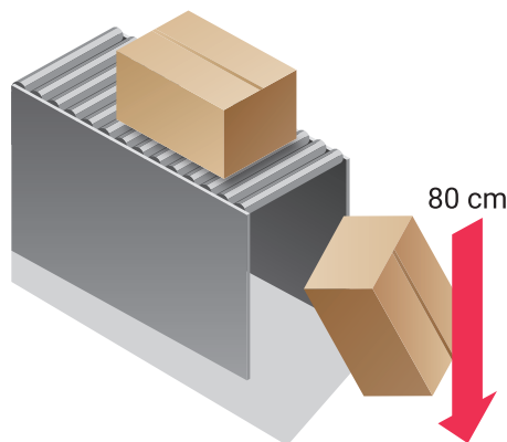
The falling crash test: free fall from 60-80 cm for weight 0-30 kg (ČSN EN 22248 and ČSN EN ISO 24180-20)
